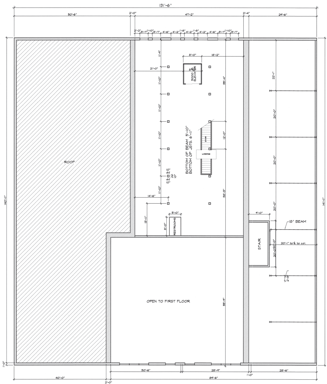
2 SECOND FLOOR PLAN SCALE: 1/8" = 1'-0"
