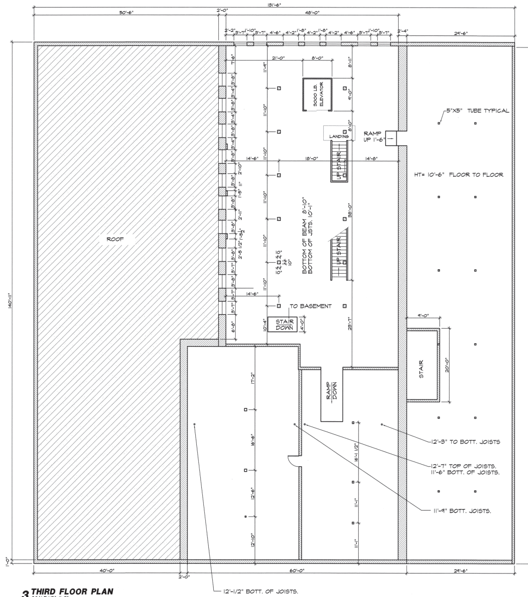
3 THIRD FLOOR PLAN SCALE: 1/8" = 1'-0"
